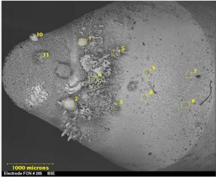
Tungsten Bearding SEM Results
