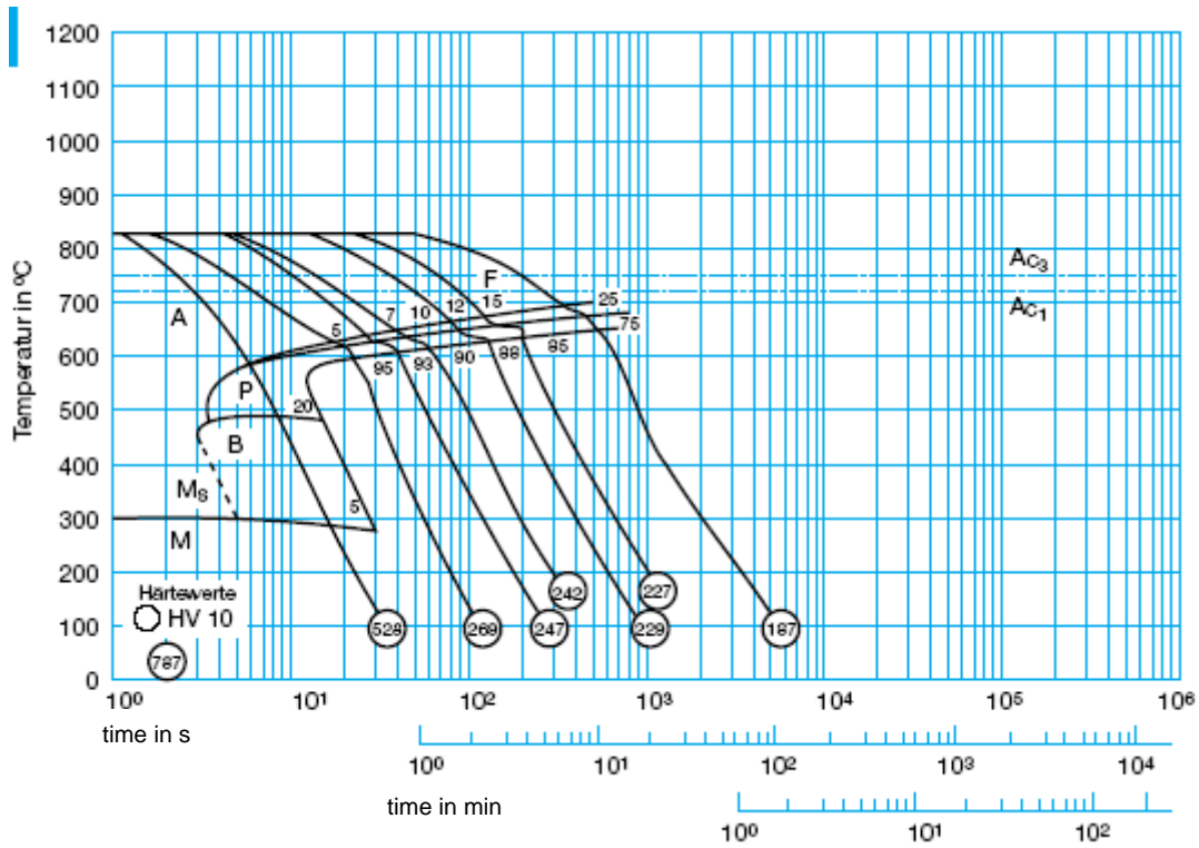
Continuously TTT-diagram of C 60E (Ck60)
