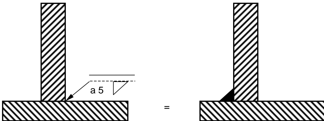
d. Single Side Fillet Weld (Different symbol representation but equivalent in practical welding execution, see also sketch "b").
