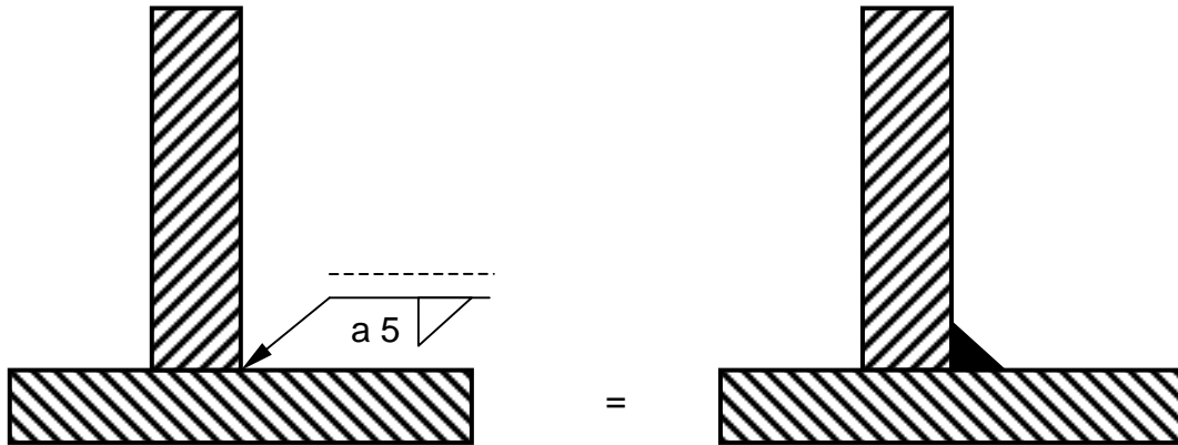
c. Single Side Fillet Weld (Different symbol representation but equivalent in practical welding execution, see also sketch "a").
