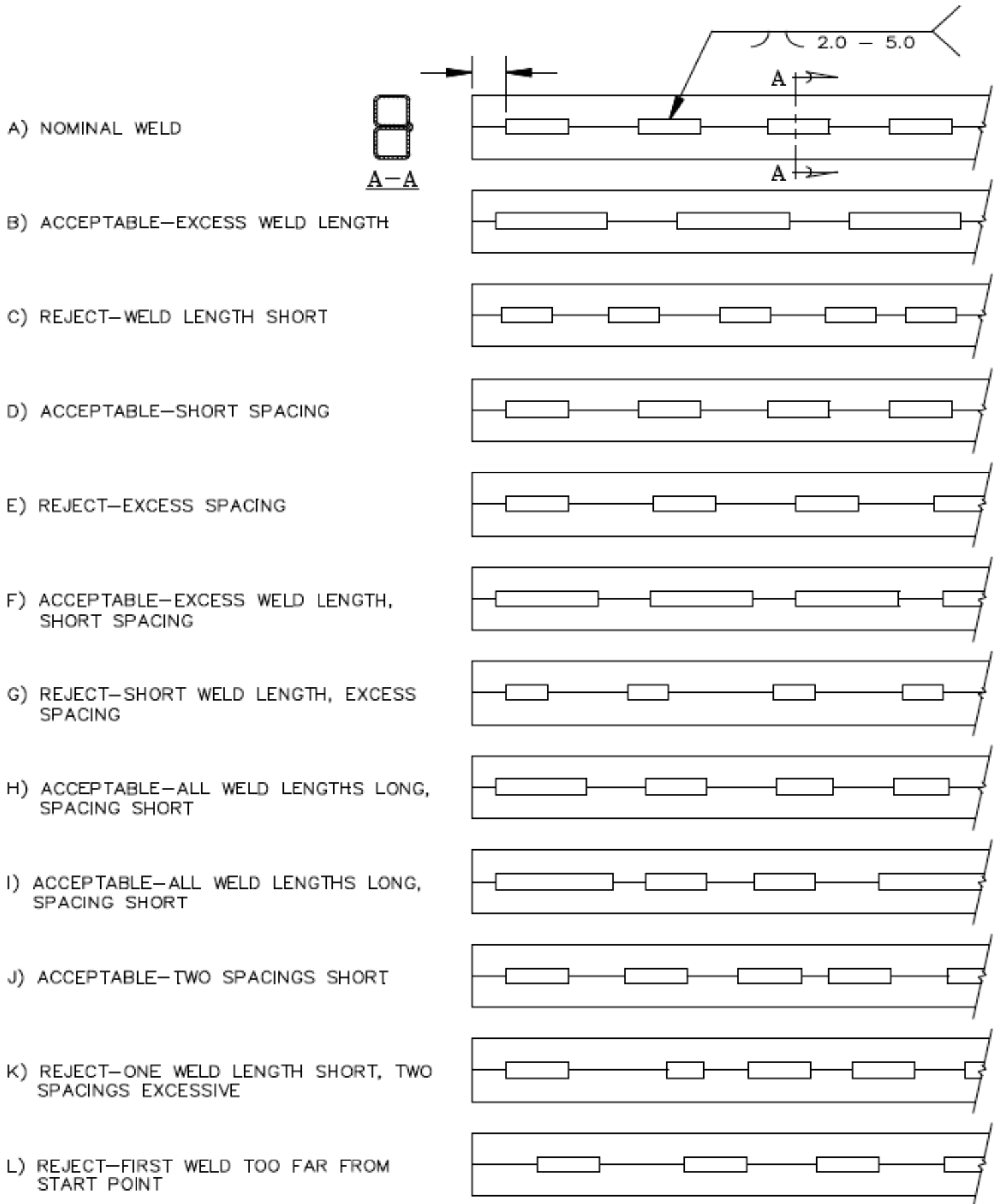
EXAMPLES OF ACCEPTABLE AND UNACCEPTABLE INTERMITTENT WELDS FOR THE WELD SYMBOL STATED
