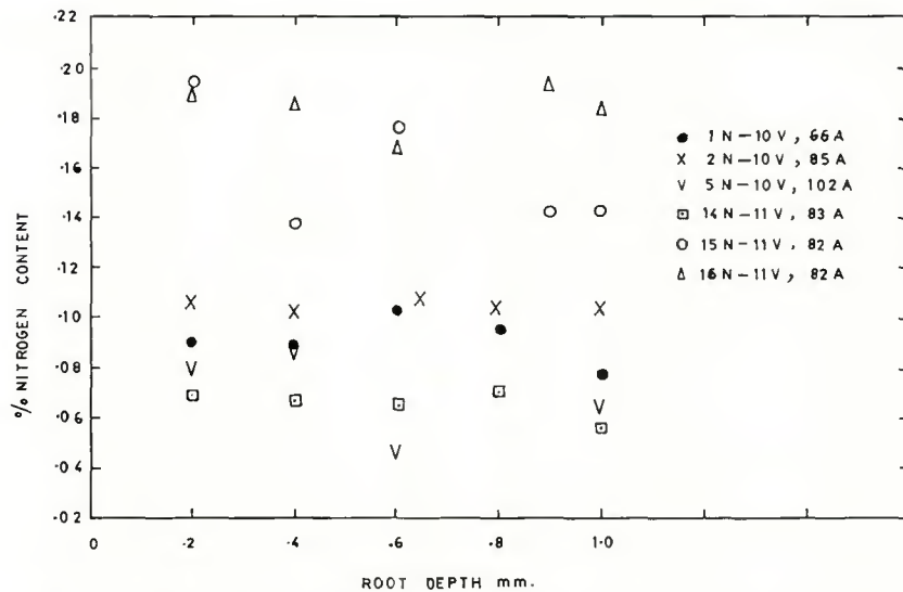
Fig. 2(a) — Nitrogen content variations in weld root passes for six nitrogen purged joints
