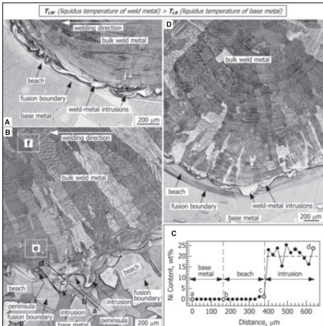
Fig. 7 — A new type of macrosegregation discovered in the present study, that is, filler-deficient beach along fusion boundary with weld metal intruding into the beach: A, B — longitudinal micrographs; C — composition profile along \underline{ad} in B; D — transverse micrograph. Compositions in area e, in area f, and along \underline{cd} all about Cu-20Ni. Base metal: pure Cu; filler metal: Cu-30Ni.
