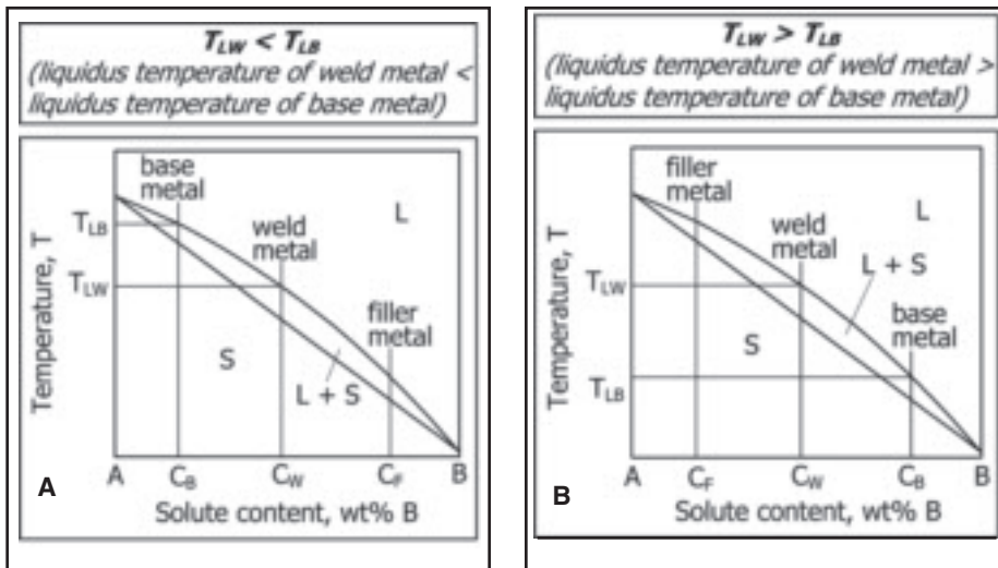
Fig. 1 — Schematic phase diagrams showing the following: A — filler metal that makes T_{LW} < T_{LB} ; B — filler metal that makes T_{LW} > T_{LB} .
