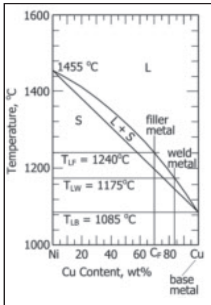
Fig. 8 — Ni-Cu phase diagram (Ref. 25) showing the liquidus temperatures of base metal T_{LB} , weld metal T_{LW} , and filler metal T_{LF} of the Cu weld made with filler metal Cu-30Ni shown in Fig. 7B.
