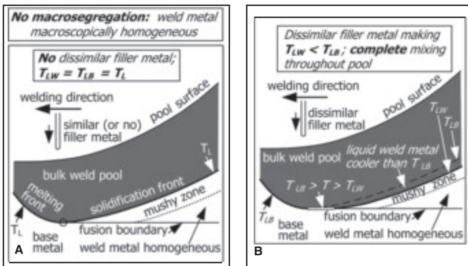
Fig. 2 — Absence of macrosegregation: A — No dissimilar filler metal; B — dissimilar filler metal makes T_{LW} < T_{LB} but mixing is complete throughout the weld pool. Pool boundary is melting front before circle and solidification front after.
