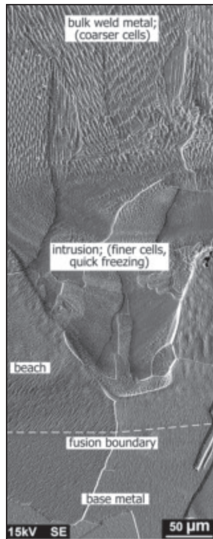
Fig. 9 — Evidence of quick freezing of intrusion in cooler layer of liquid base metal suggested by Mechanism 2. SEM image (of intrusion intersected by \underline{cd} in Fig. 7B) shows much finer cells in intrusion than in nearby bulk weld metal of same composition. Base metal: pure Cu; filler metal: Cu-30Ni.
