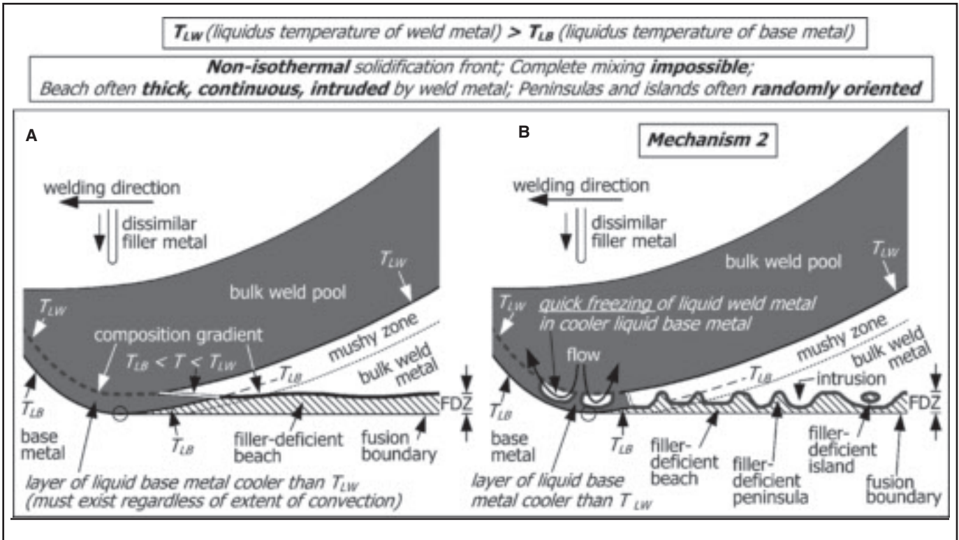
Fig. 6 — Formation of fusion-boundary macrosegregation (filler-deficient zone FDZ) when filler metal makes T_{LW} > T_{LB} : A — beach; B — weld-metal intrusions, beach, peninsulas, and islands by Mechanism 2. Pool boundary is melting front before circle and solidification front after.
