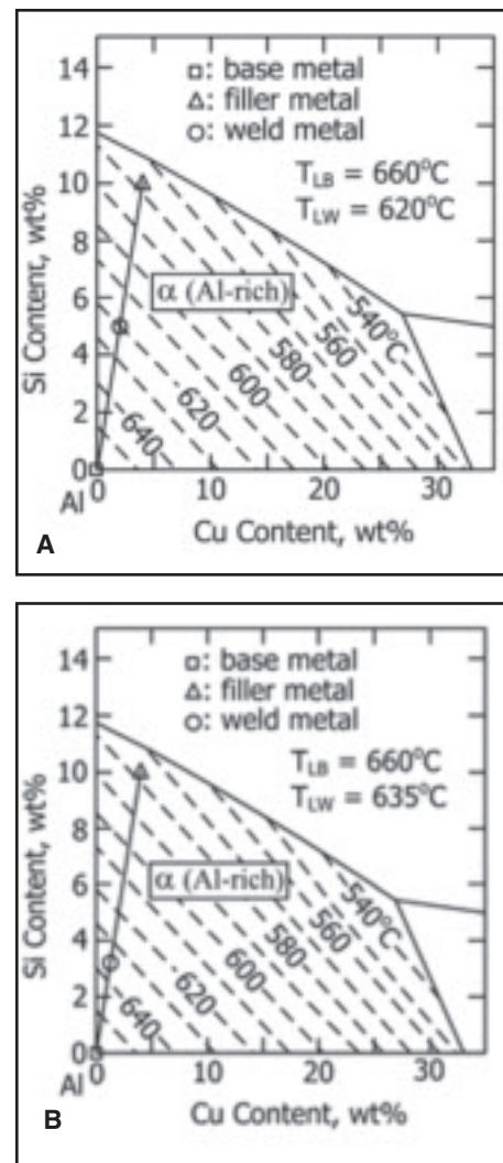
Fig. 5 — Liquidus projection of ternary Al-Cu-Si system showing liquidus temperatures of base metal T_{LB} and weld metal T_{LW} for welds of 1100 Al (pure Al) made with filler 4145 Al (Al-4Cu-10Si): A — welds shown in Fig. 4A-C (50% dilution); B — weld shown in Fig. 4D-F (68% dilution).
