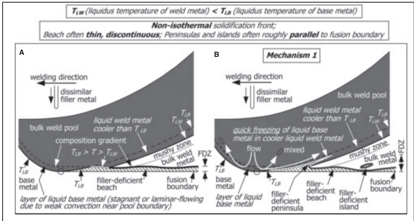
Fig. 3 — Formation of fusion-boundary macrosegregation (filler-deficient zone FDZ) when filler metal makes T_{LW} < T_{LB} : A — beach; B — beach, peninsula, and island by Mechanism 1. Pool boundary is melting front before circle and solidification front after.
